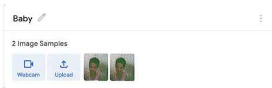
Figure 4.5: Class 1
