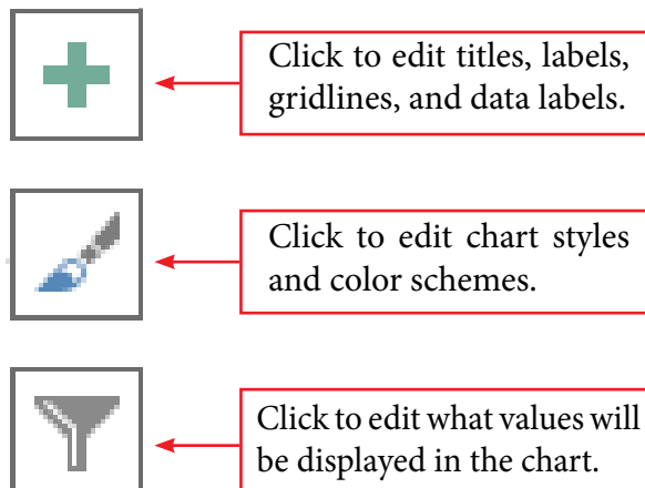
Figure 1.4: Chart Elements
