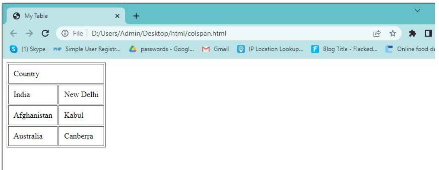
Figure 6.5: Colspan
