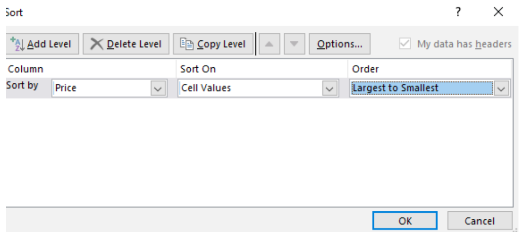
Figure 1.10: Sort
