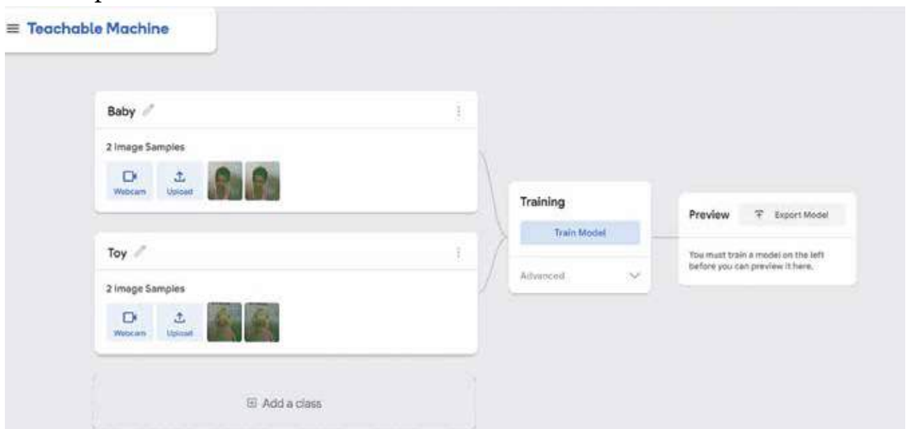
Figure 4.4: Creating Samples
