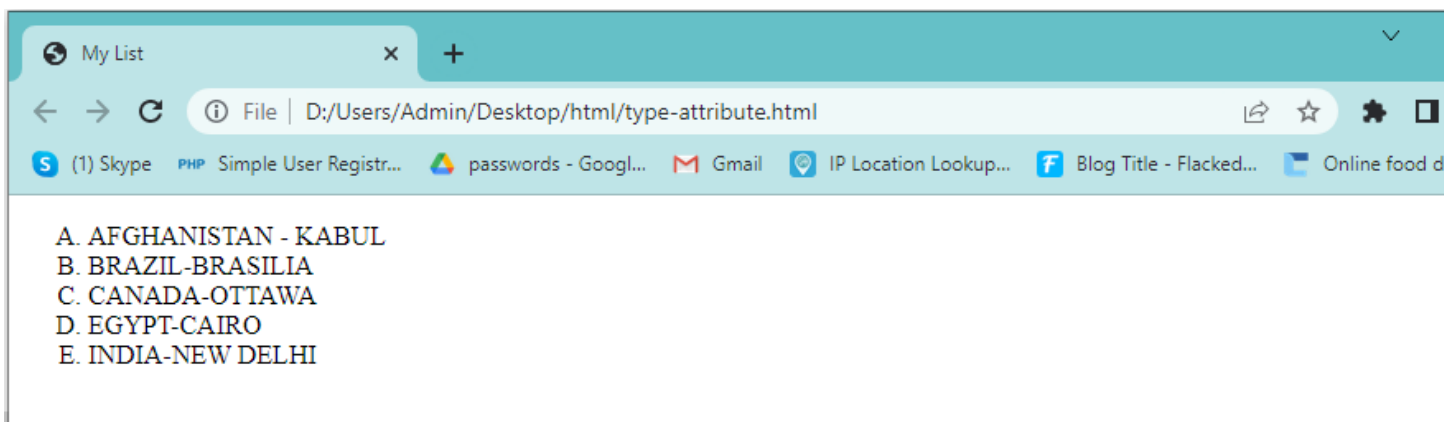
Figure 6.10: Type Attribute
