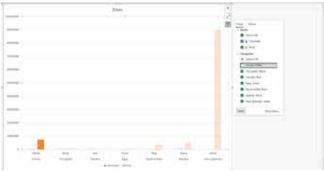
Figure 1.5: Chart Filters
