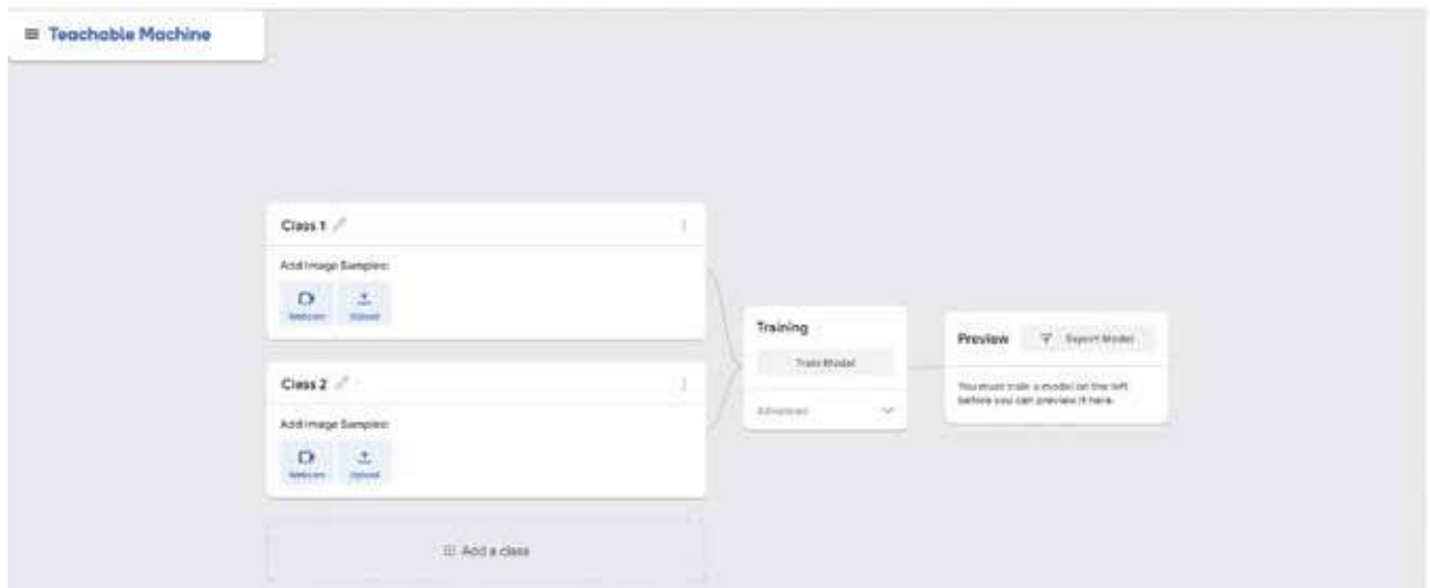
Figure 4.3: Creating Project
