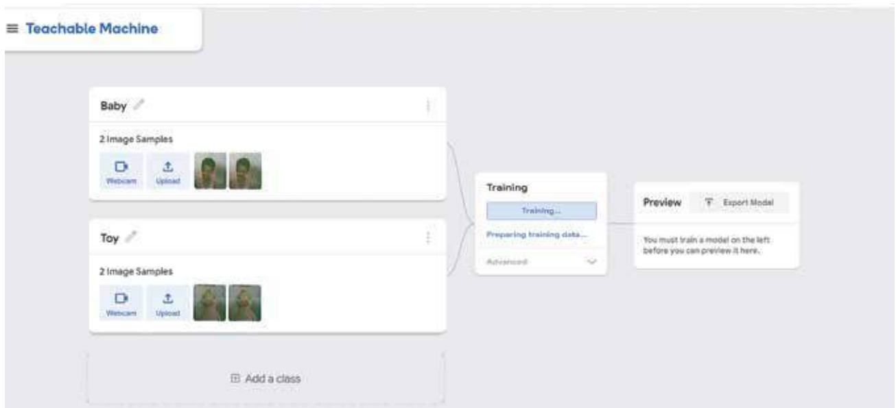
Figure 4.7: Model Training
