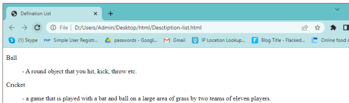
Figure 6.13: Description List
