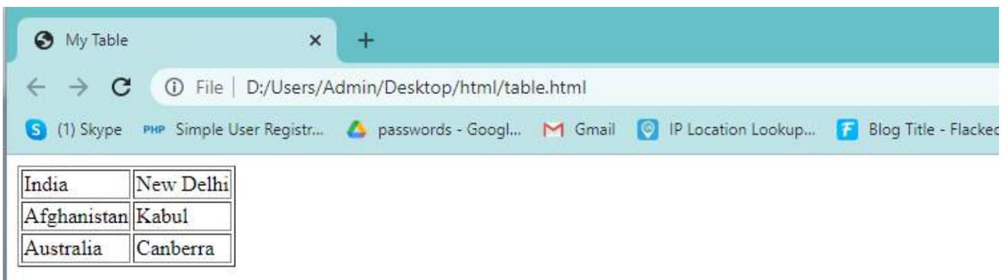
Figure 6.2: Border Attribute
