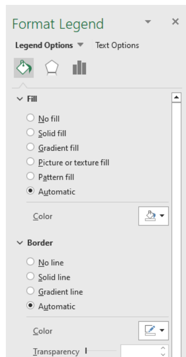
Figure 1.8: Format Legend
