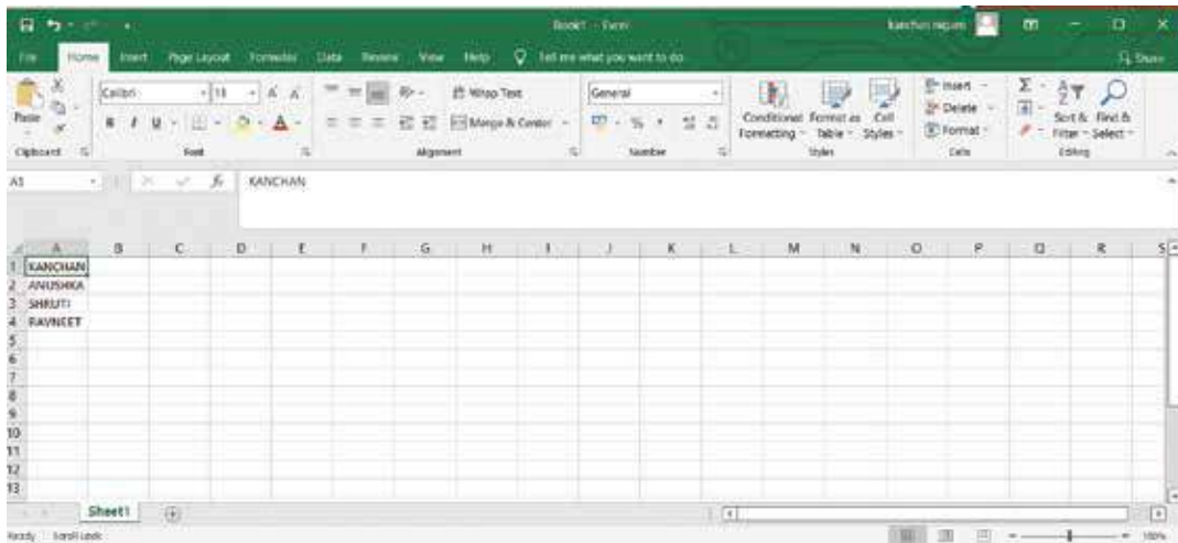
Figure 3.3 Ready Mode
