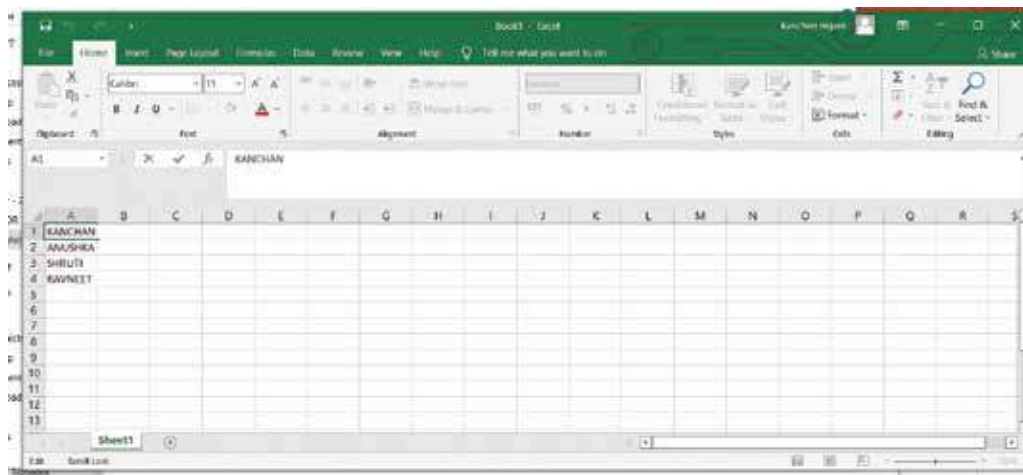
Figure 3.4 Edit Mode.
