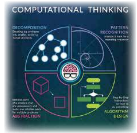
Figure 5.1 Computational Thinking
